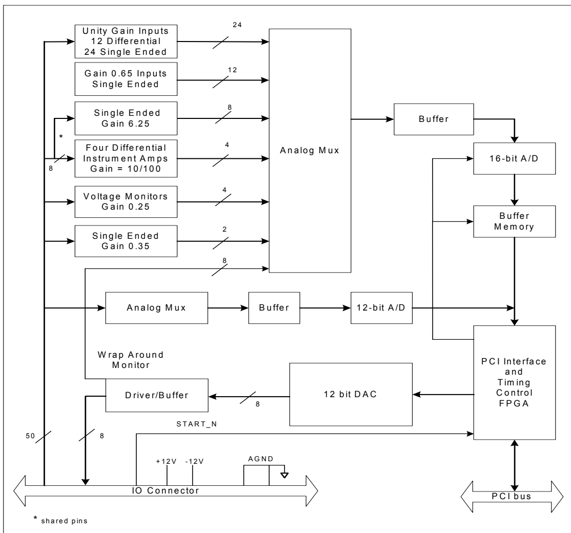
M453 Block Diagram
